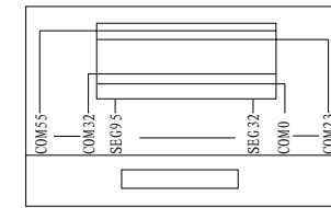
COM&SEG LAYOUT
