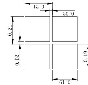
Detail A (20:1)
